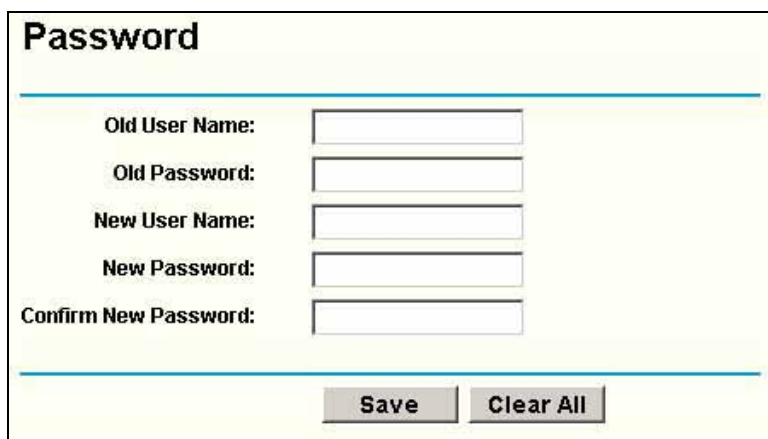
Figure 5-42: Password
